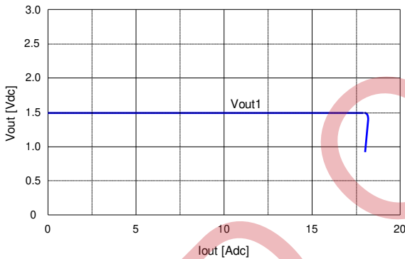
Figure 25. Output voltage Vout1 vs. load current lout1 showing current limit point and converter shutdown point. When Vout1 is in current limit, Vout2 is not affected until Vout1 reaches the shut-down threshold of 60% of its nominal value. Input voltage has almost no effect on Vout1 current limit characteristic.
