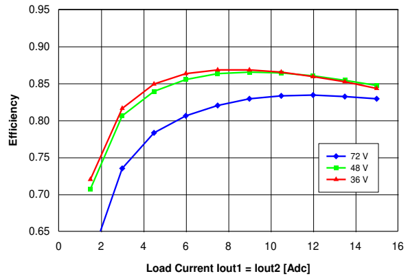
Figure 16. Efficiency vs. balanced load current ( I_{out1} = I_{out2} ) and input voltage for converter mounted horizontally with air flowing from pin 3 to pin 1 at a rate of 300 LFM (1.5 m/s) and T_a = 25 °C.
