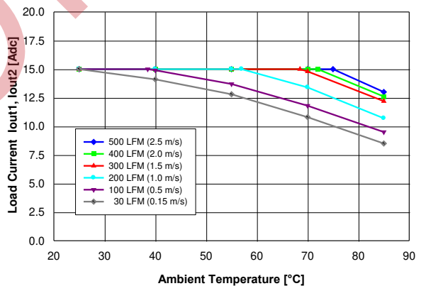
Figure 10. Available balanced load current ( i_{out1} = i_{out2} ) vs. ambient temperature and airflow rates for converter with D height pins mounted horizontally with V_{in} = 48 V, air flowing from pin 3 to pin 1 and maximum FET temperature \leq 120 °C.
