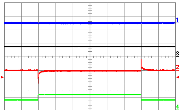
Figure 22. Output voltage response to lout2 load current step-change of 3.75 A (50%-75%-50%) at lout1 = 7.5 A and V_{in} = 48\text{ V} . Ch1 = Vout1 (100 mV/div), Ch2 = Vout2 (100 mV/div), Ch3 = lout1 (10 A/div.), Ch4 = lout2 (10 A/div.). Current slew rate: 5 A/ \mu\text{s} , C_o = 300\text{ }\mu\text{F} tantalum + 1 \mu\text{F} ceramic. Time scale: 0.5 ms/div.
