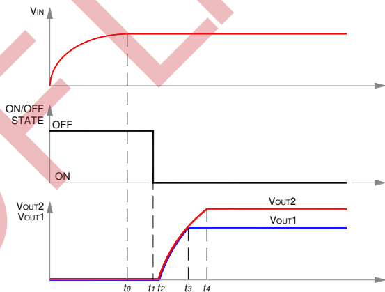
Figure 5. Startup scenario #2.
