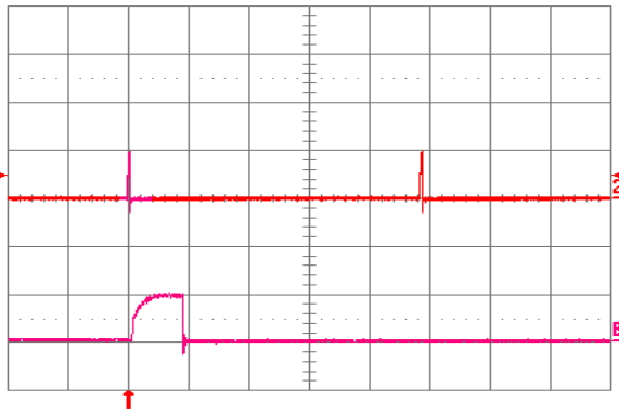
Figure 29. Load current I_{out1} into a 10\text{ m}\Omega short circuit on V_{out1} during re-start, with V_{out2} open (no load), at V_{in} = 48\text{ V} . Ch2 = I_{out1} (20 A/div, 20 ms/div). ChB = I_{out1} (20 A/div, 1 ms/div) is an expansion of the on-time portion of I_{out1} .
