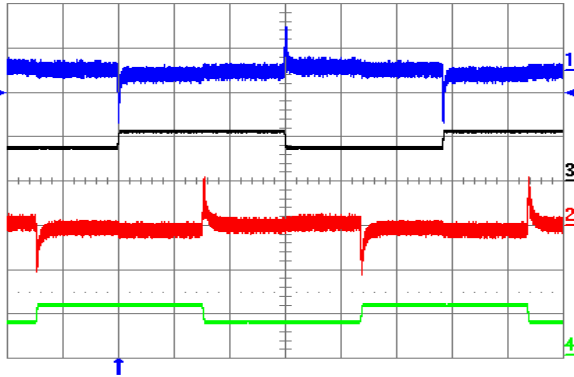
Figure 23. Output voltage response to both lout1 and lout2 (out of phase) load current step-change of 3.75 A (50%-75%-50%) at V_{in} = 48 V. Ch1 = Vout1 (50 mV/div), Ch2 = Vout2 (50 mV/div), Ch3 = lout1 (10 A/div.), Ch4 = lout2 (10 A/div.). Current slew rate: 0.1 A/ \mu s, C_o = 10 \mu F tantalum + 1 \mu F ceramic. Time scale: 1.0 ms/div.
