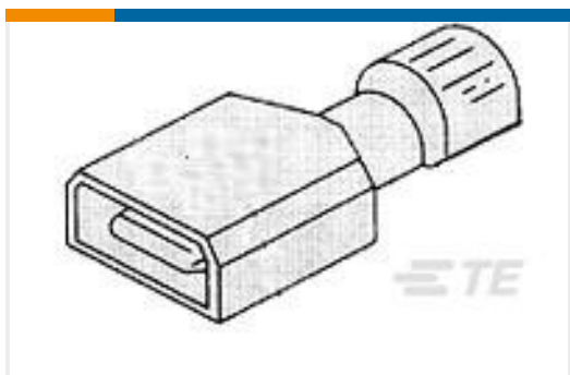
TE Part #2-521192-2 ULTRA-FAST 250 ASY REC 22-18 TPBR
