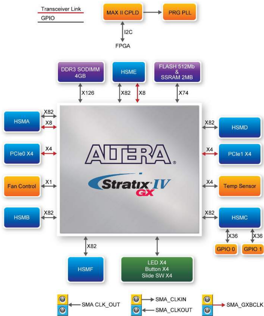
Figure 1-3 TR4 Block Diagram
