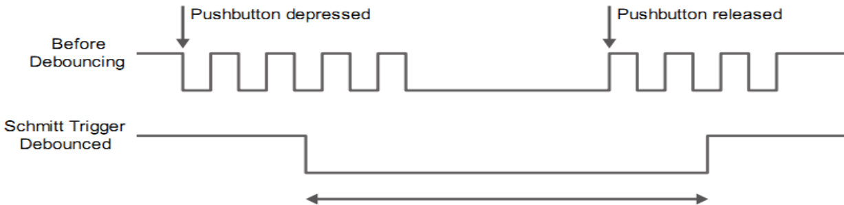
Figure 2-10 Push-button Debouncing
