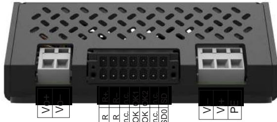
Fig. 12 Pin allocation of RCM150
