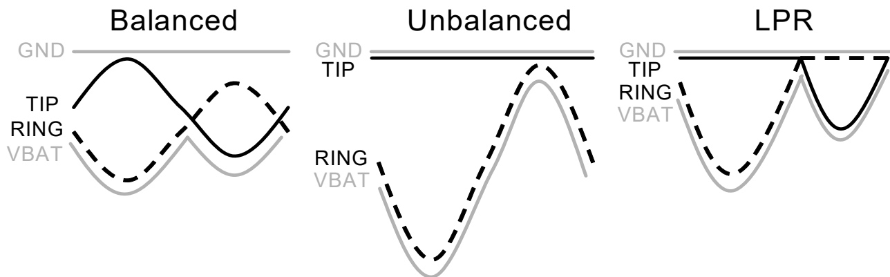
Figure 21. Ringing Modes
