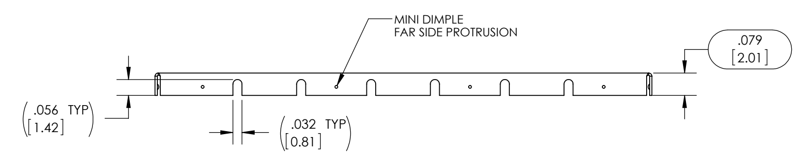
FORMED COVER
