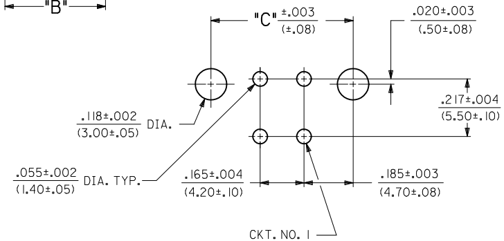
RECOMMENDED HOLE LAYOUT FOR .070/(1.78) MAX. THICK P.C. BOARD (SEE NOTE 5)
