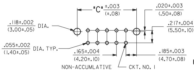
MATE-FIRST/BREAK-LAST DETAIL (SEE NOTE 12)
