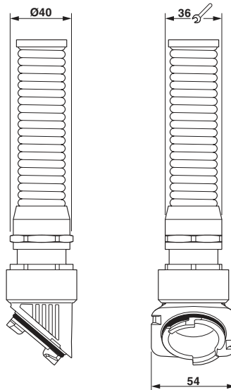
Dimensional drawing
