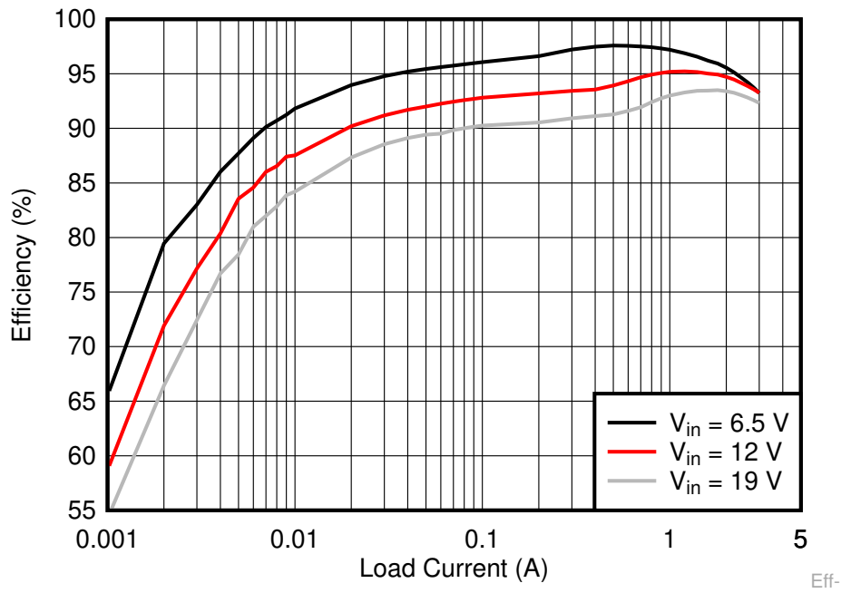
Figure 5-1. TPS56339EVM Efficiency
