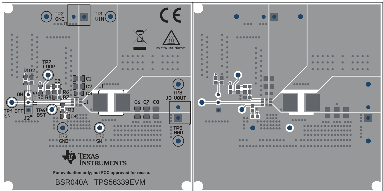
Figure 6-1. Top Assembly
