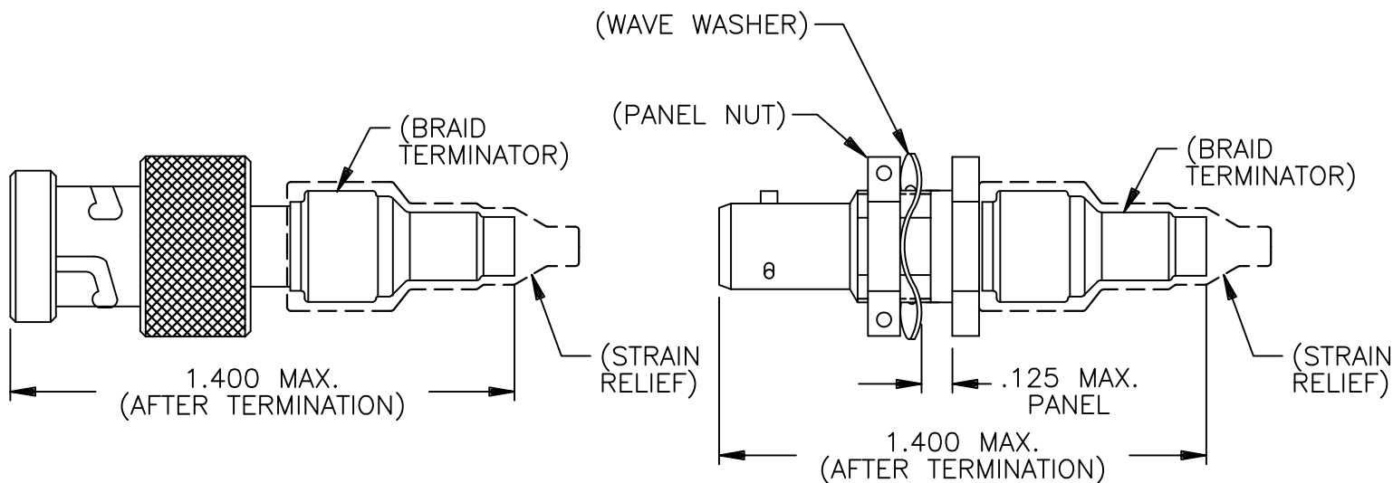
JACK CONNECTOR ASSEMBLY
