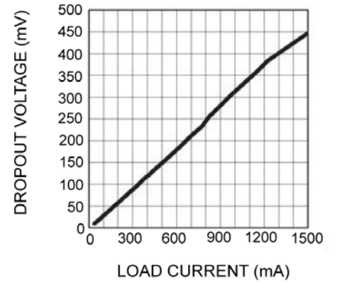
Six Parallel Current Sink Dropout vs. Load Current
