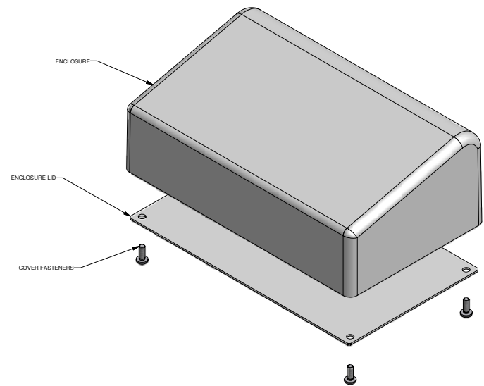
ENCLOSURE ASSEMBLY
