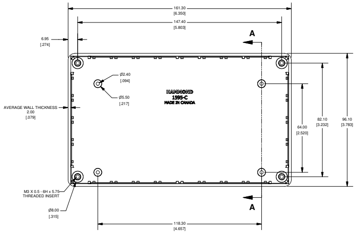
ENCLOSURE
