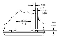
DETAIL B SCALE 1.50 : 1
