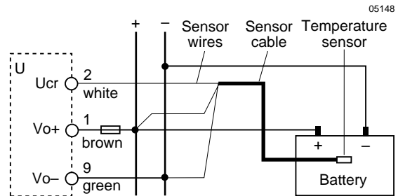
Fig. 4: Connection to the U unit.
