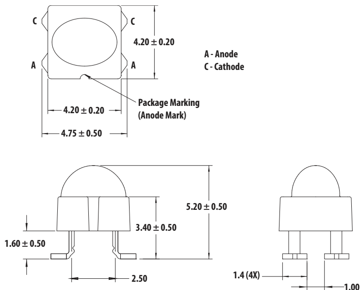
Figure 1: Package Dimensions
