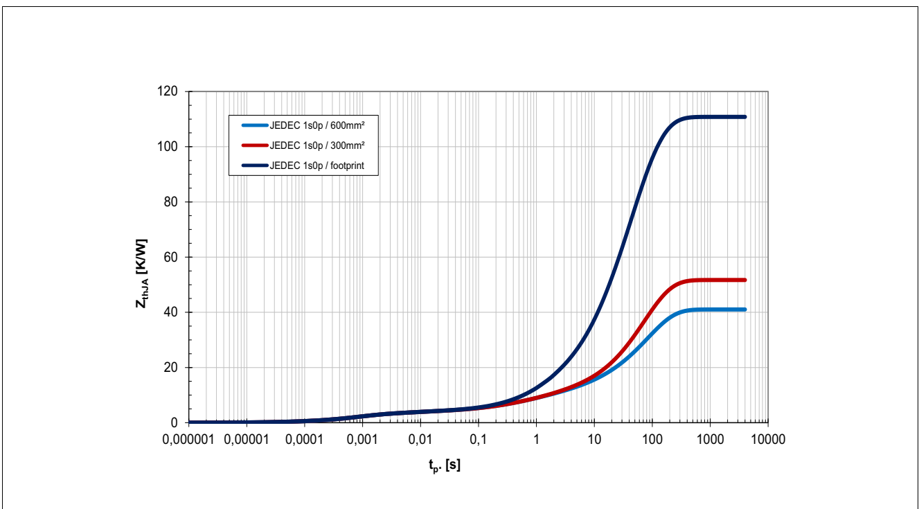
Figure 8 Typical transient thermal impedance Z_{thJA} = f(t_p) , T_a = 85^\circ\text{C} Value is according to Jeduc JESD51-3 at natural convection on FR4 1s0p board. Device is dissipating 1 W power.
