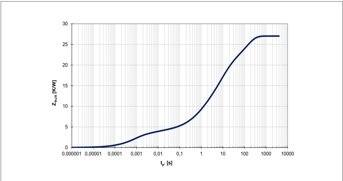
Figure 7 Typical transient thermal impedance Z_{thJA} = f(t_p) , T_A = 85^\circ\text{C} Value is according to Jeduc JESD51-2,-7 at natural convection on FR4 2s2p board; The product (Chip+Package) was simulated on a 76.2 \times 114.3 \times 1.5 \text{ mm}^3 board with 2 inner copper layers (2 x 70 \mu\text{m} Cu, 2 x 35 \mu\text{m} Cu). Device is dissipating 1 W power.
