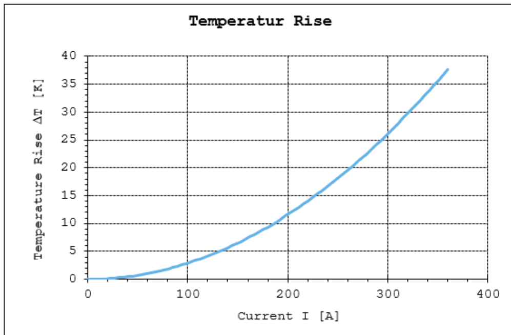
Figure 1. Current &amp; Temperature-rise Curve of TE Crown Clip Junior HC320 Power Connector 2204900
