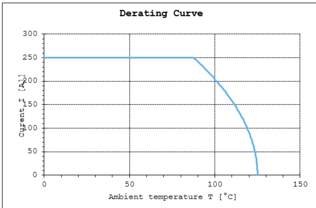
Figure 4. Derating Curve of TE Crown Clip Junior HC250 Power Connector 2204899
