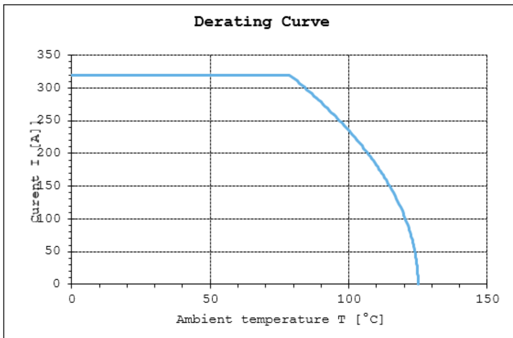
Figure 3. Derating Curve of TE Crown Clip Junior HC320 Power Connector 2204900
