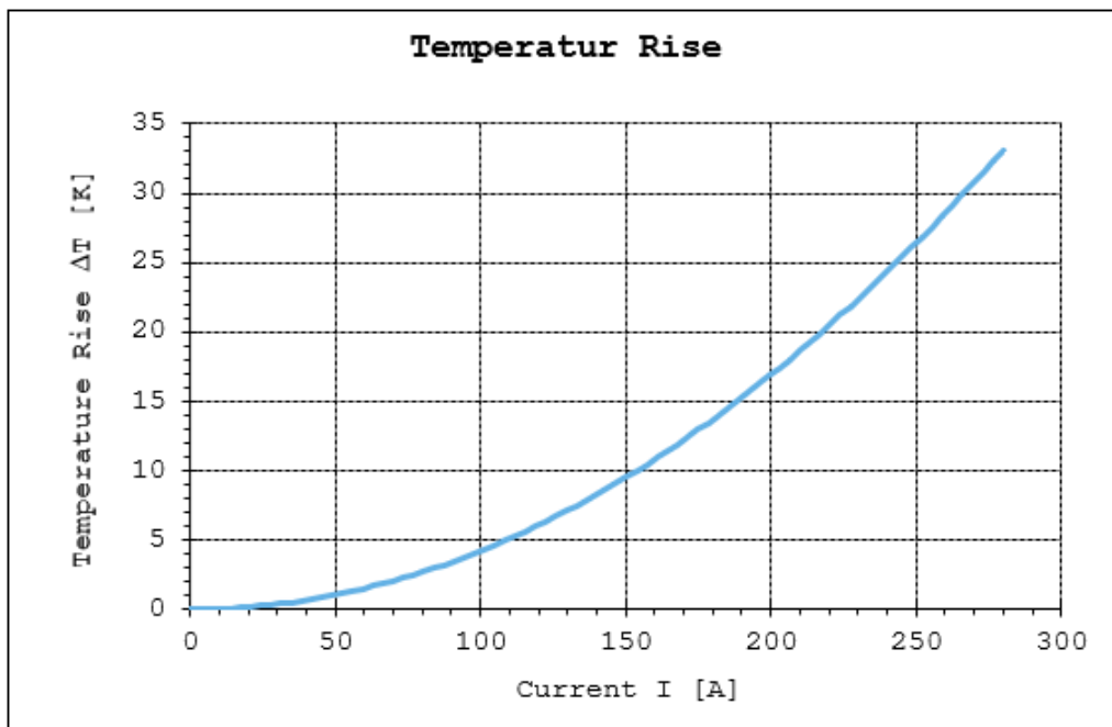
Figure 2. Current &amp; Temperature-rise Curve of TE Crown Clip Junior HC250 Power Connector 2204899
