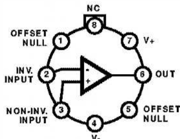
CA741, CA741C, LM741, LM741C (PDIP) TOP VIEW
