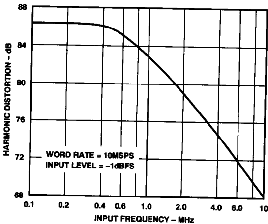
Figure 1. Harmonic Distortion vs. Analog Input
