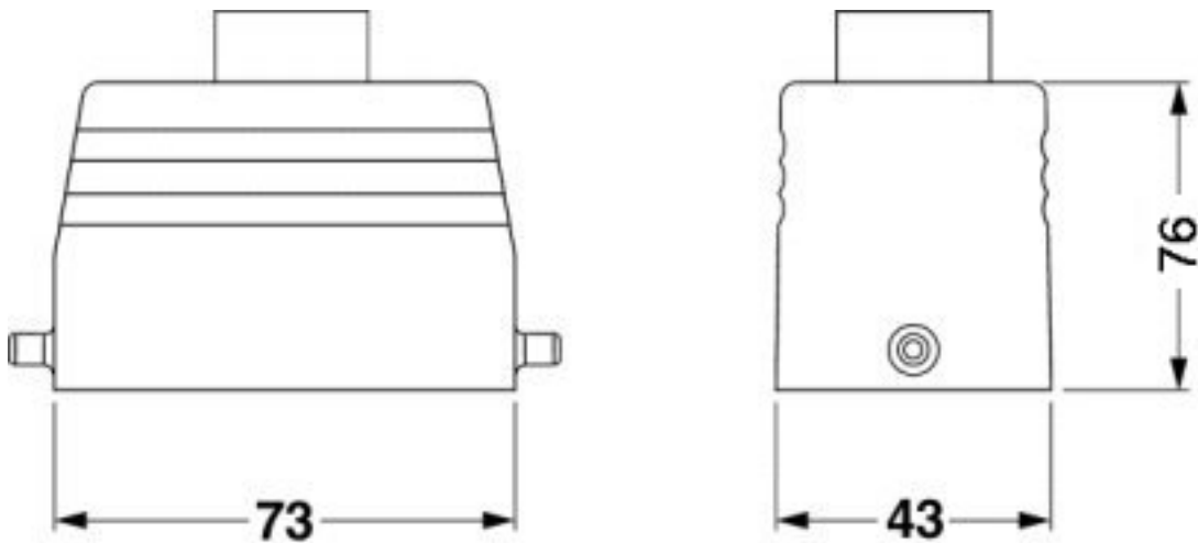
Dimensioned drawing
