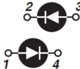
Figure 2 • Anti-parallel MSC2X50SDA070J
