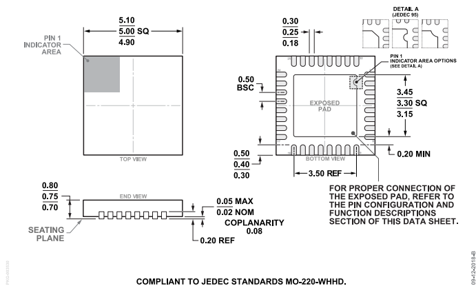
COMPLIANT TO JEDEC STANDARDS MO-220-WHHD. Figure 43. 32-Lead Lead Frame Chip Scale Package [LFCSP] 5 mm × 5 mm Body and 0.75 mm Package Height (CP-32-13) Dimensions shown in millimeters
