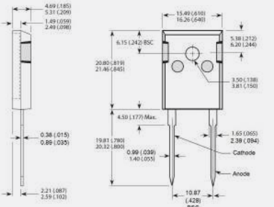
TO-247 2-Lead
