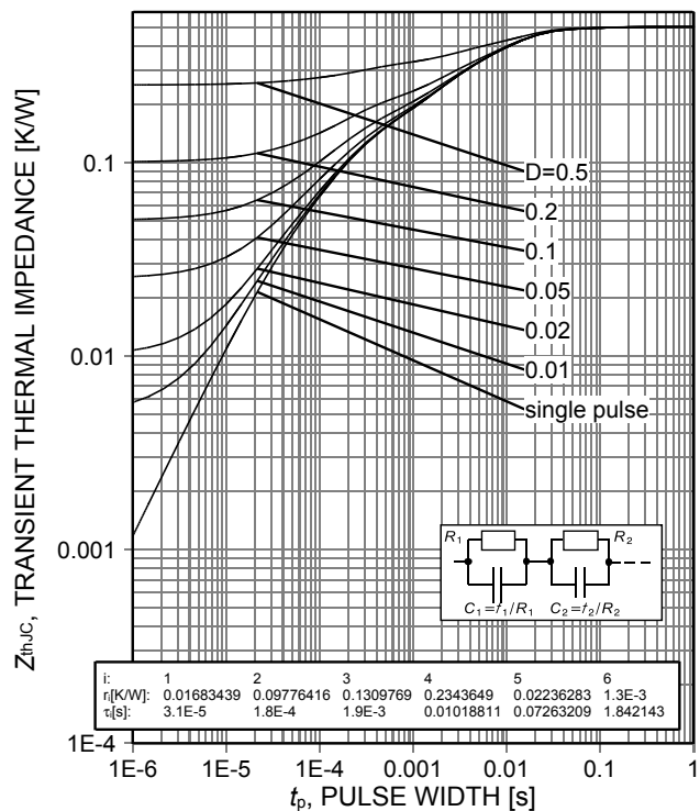
Figure 20. Typical IGBT transient thermal impedance ( D = t_p / T )
