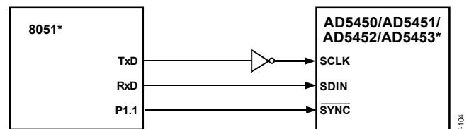
Figure 57. 80C51/80L51-to-AD5450/AD5451/AD5452/AD5453 Interface
