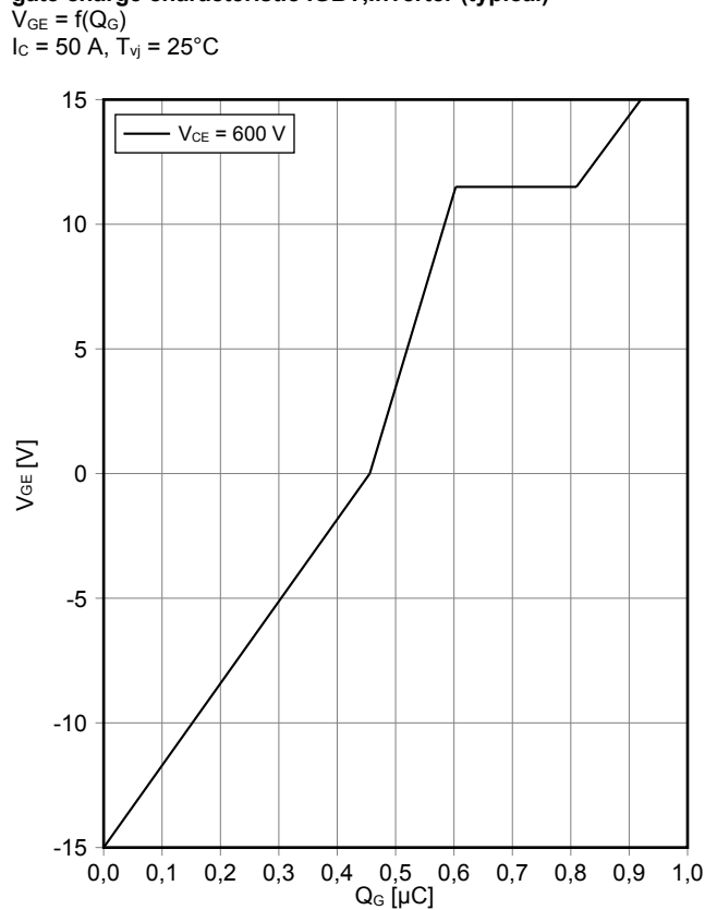
Gateladungs Charakteristik IGBT, Wechselrichter (typisch) gate charge characteristic IGBT, Inverter (typical) V_{GE} = f(Q_G) I_C = 50\text{ A} , T_{vj} = 25^\circ\text{C}
