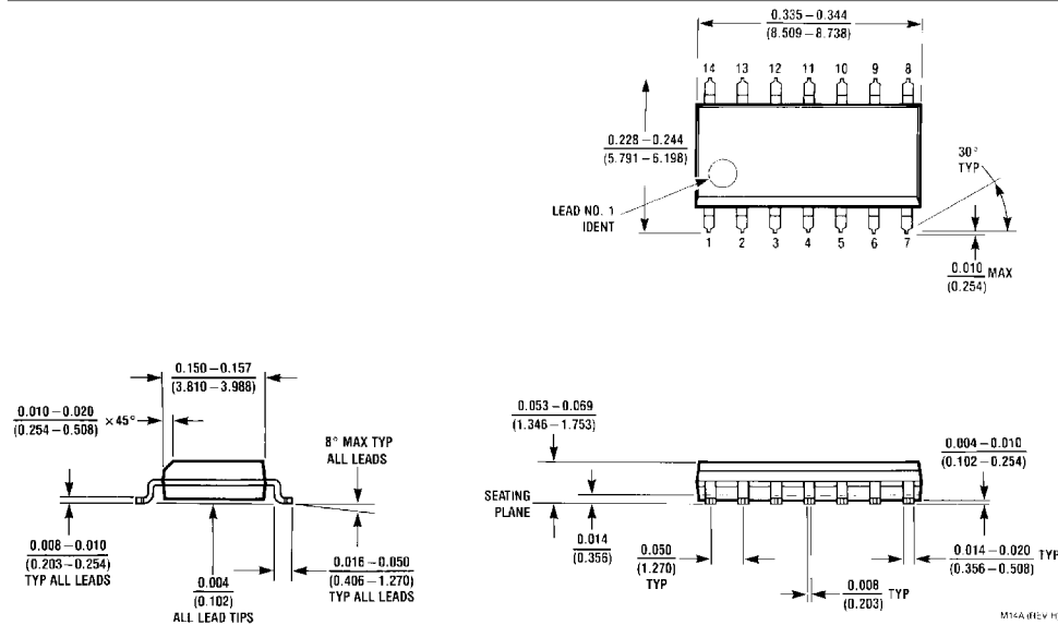
14-Lead Small Outline Molded Package (M) Order Number DM74LS04M NS Package Number M14A
