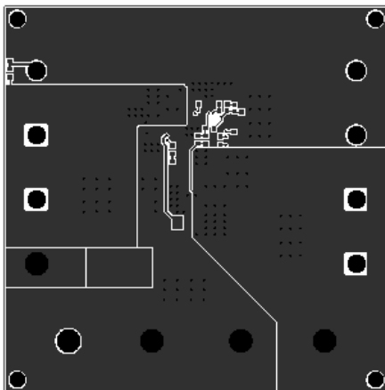
Figure 3: Bottom Layer
