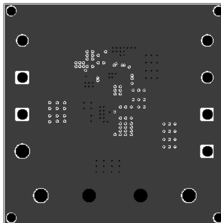
Figure 5: Inner Layer 2
