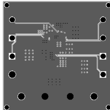
Figure 4: Inner Layer 1
