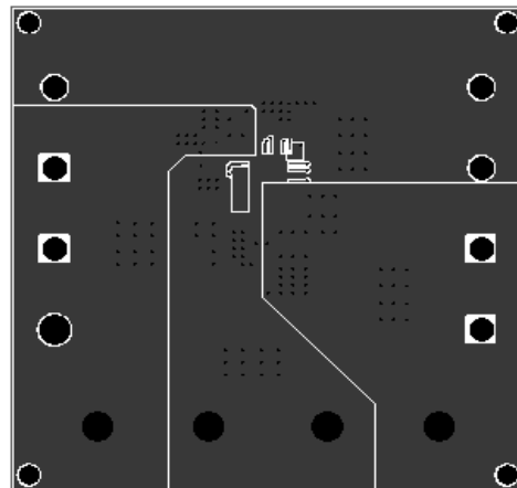
Figure 2: Top Layer
