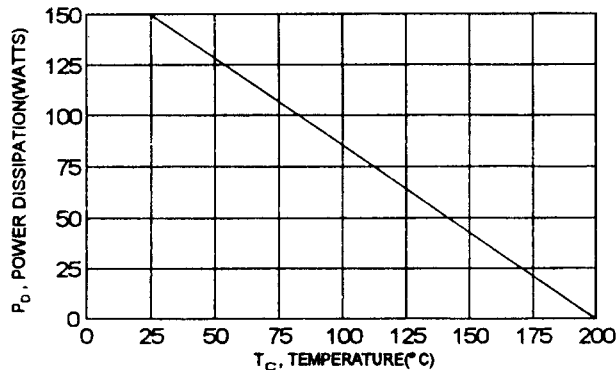
FIGURE -1 POWER DERATING
