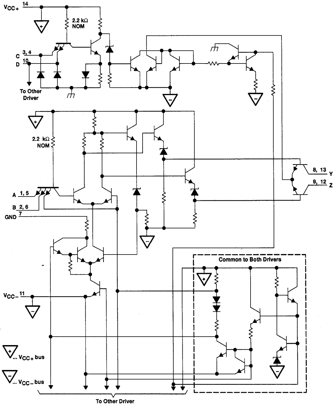
schematic (each driver)
