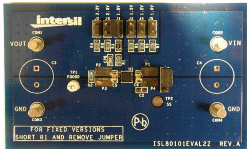
FIGURE 1. ISL80101EVAL2Z
