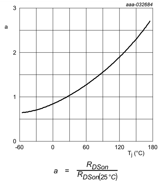
Fig. 8. Normalized drain-source on-state resistance as a function of junction temperature
