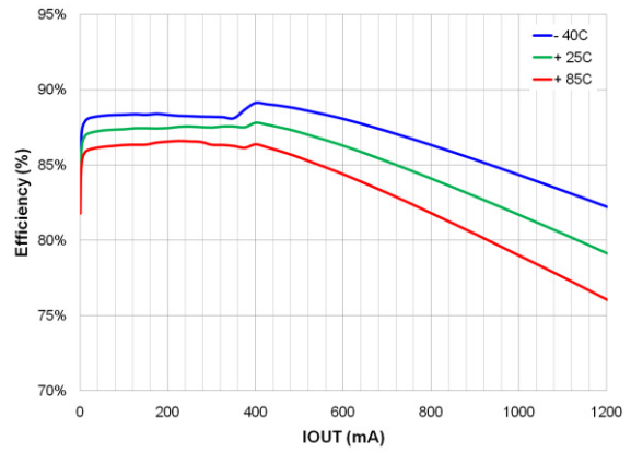
Figure 5. Efficiency vs. Load Current and Temperature
