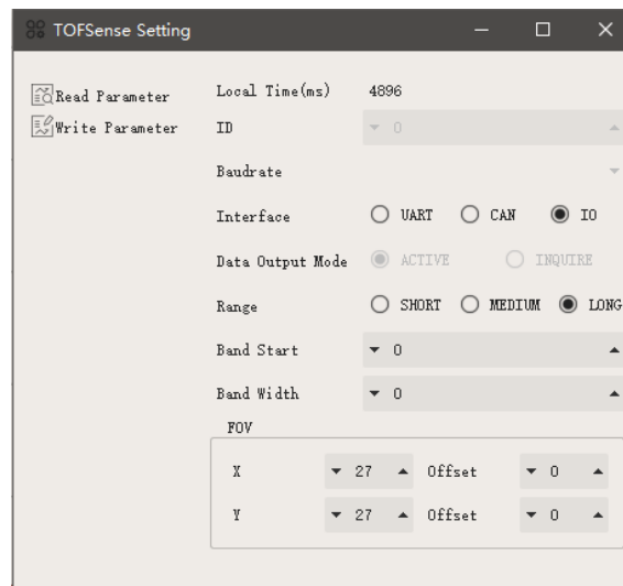
Figure 5: I/O Output Mode Configuration Diagram
