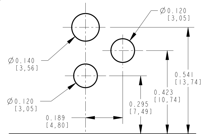
ALTERNATE PC BOARD LAYOUT (COMPONENT SIDE)
