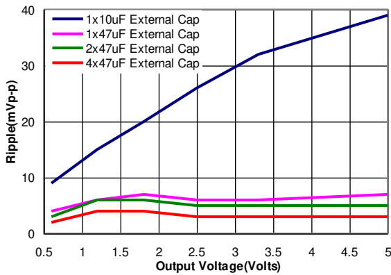
Figure 47. Output ripple voltage for various output voltages with external 1x10 μF, 1x47 μF, 2x47 μF or 4x47 μF ceramic capacitors at the output (3A load). Input voltage is 12V.
