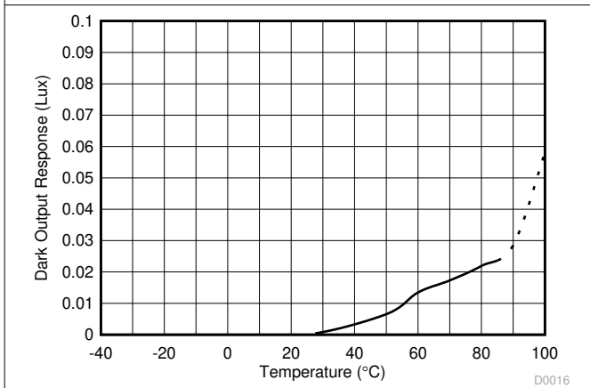
Figure 7-10. Dark Response vs Temperature
