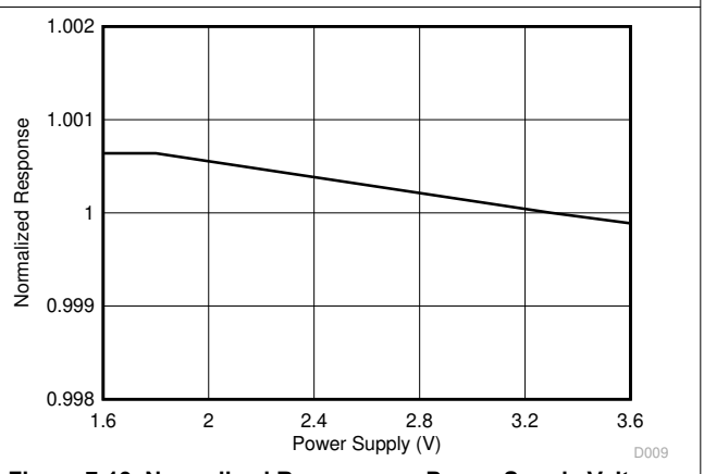
Figure 7-13. Normalized Response vs Power-Supply Voltage
