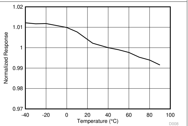
Figure 7-11. Normalized Response vs Temperature
