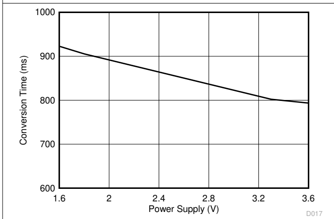
Figure 7-12. Conversion Time vs Power Supply
