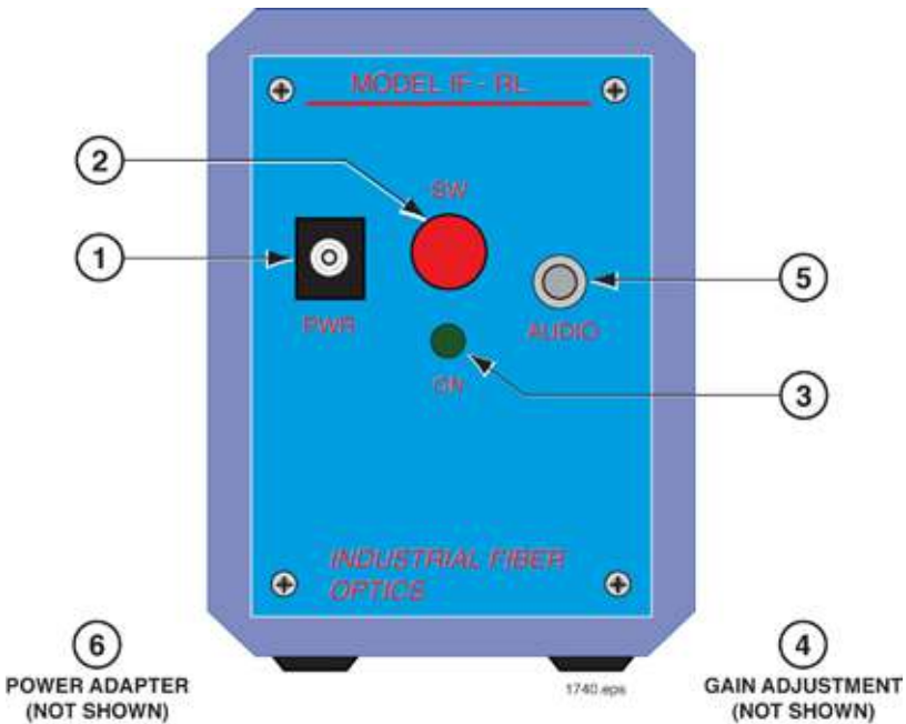
Figure 1. Rear view of laser showing electrical inputs and controls.
