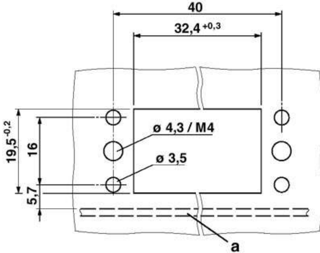
Dimensioned drawing
