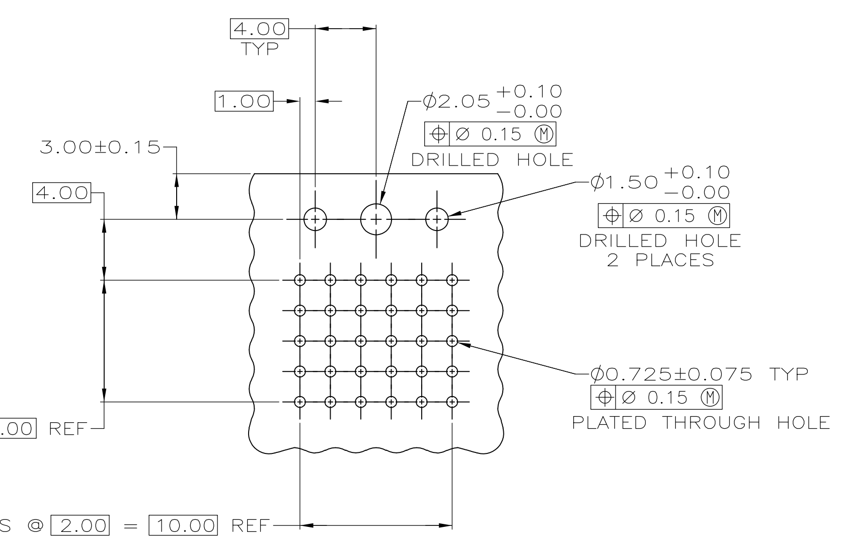
RECOMMENDED CIRCUIT PATTERN PER IPC-D300 TYPE II, CLASS 3 COMPONENT SIDE
