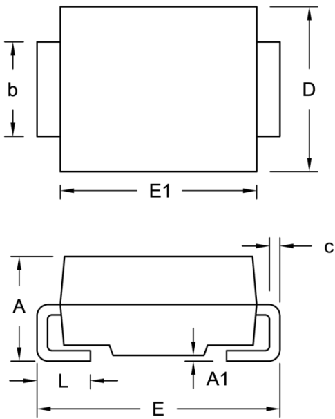
DO-214AA (SMB)
