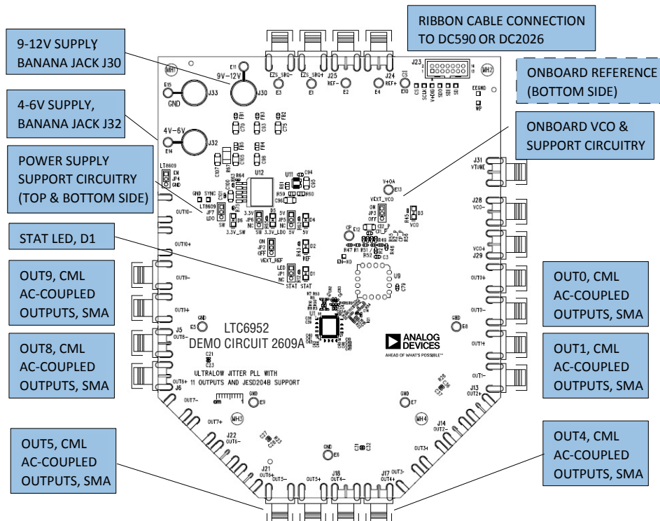
Figure 1. DC2609A Connections
