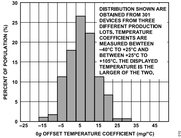
Figure 19. X-Axis 0 g Offset Temperature Coefficient (mg/°C), V_S = 3.3 V
