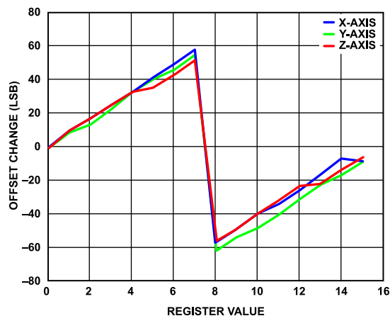
Figure 47. User Offset Trim Profile
