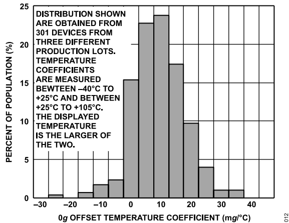
Figure 21. Z-Axis 0 g Offset Temperature Coefficient, V_S = 3.3 V
