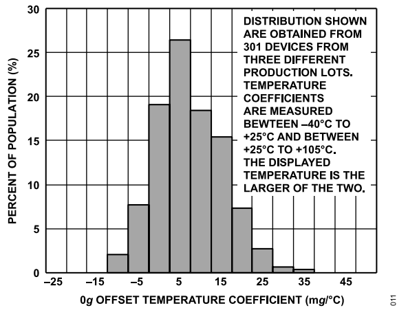
Figure 20. Y-Axis 0 g Offset Temperature Coefficient (mg/°C), V_S = 3.3 V
