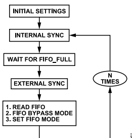
Figure 58. FIFO Workaround Implementation Example
