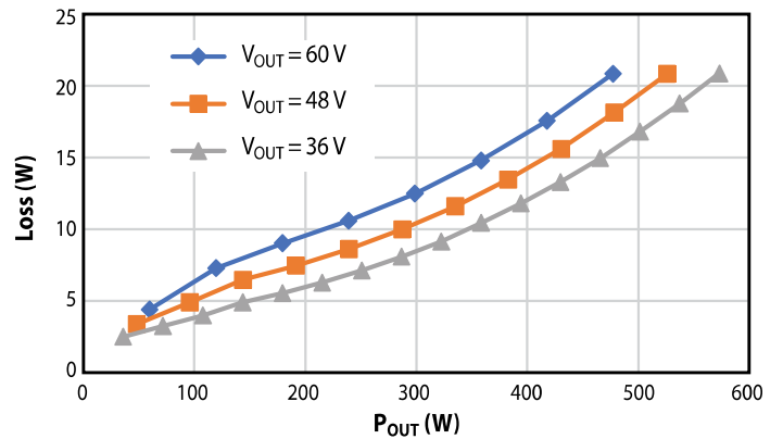
Figure 2(b): Typical losses for different output voltage (12 V input, 1000 LFM air flow)
