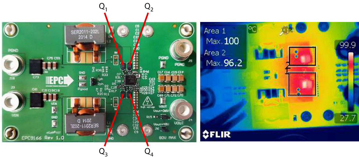
Figure 8: Typical thermal performance: V_{IN} = 12\text{ V} , V_{OUT} = 48\text{ V} , I_{OUT} = 10\text{ A} , 400 LFM air flow
