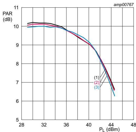
V_{DS} = 28\text{ V}; I_{Dq} = 200\text{ mA}; V_{GS(amp)peak} = 0.6\text{ V}. (1) f = 2110\text{ MHz} (2) f = 2155\text{ MHz} (3) f = 2200\text{ MHz}
