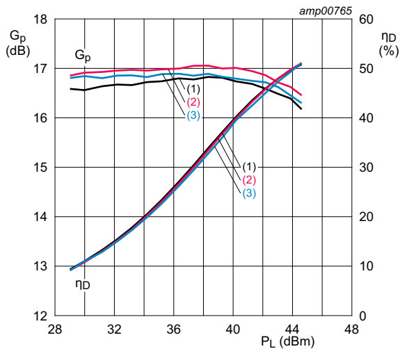
V_{DS} = 28\text{ V}; I_{Dq} = 200\text{ mA}; V_{GS(amp)peak} = 0.6\text{ V}. (1) f = 2110\text{ MHz} (2) f = 2155\text{ MHz} (3) f = 2200\text{ MHz}
