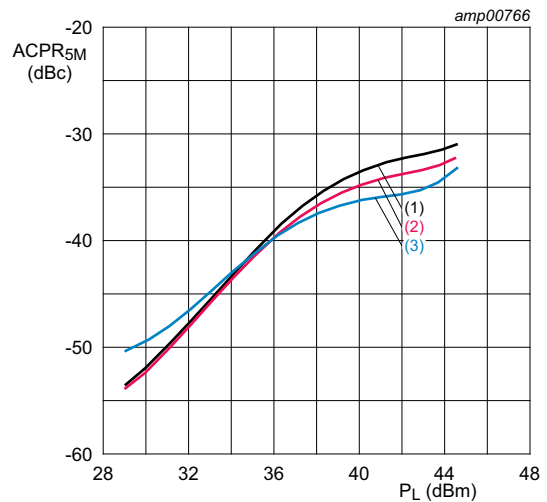
V_{DS} = 28\text{ V}; I_{Dq} = 200\text{ mA}; V_{GS(amp)peak} = 0.6\text{ V}. (1) f = 2110\text{ MHz} (2) f = 2155\text{ MHz} (3) f = 2200\text{ MHz}
