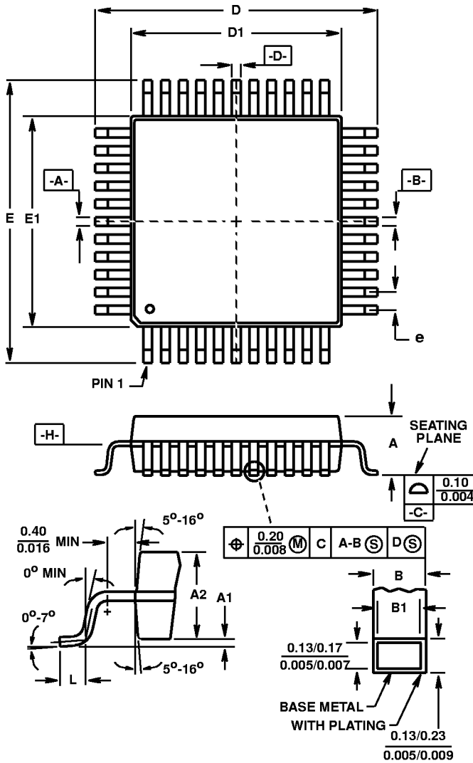
Q44.10x10 (JEDEC MO-108AA-2 ISSUE A) 44 LEAD METRIC PLASTIC QUAD FLATPACK PACKAGE
