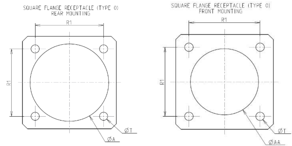
Panel Cutout
