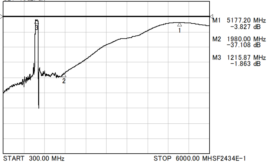
S11 5dB/div S22 5dB/div
