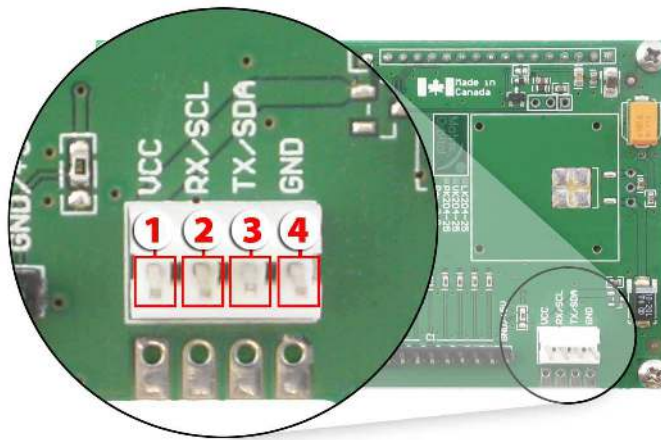
Figure 16: Power Connector and Pin out
