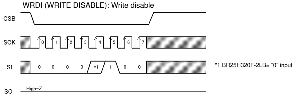
Figure 36. Write disable
