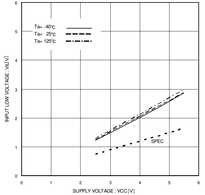
Figure 8. Input Low voltage V_{IL} (CSB,SCK,SI,HOLDB,WPB)
