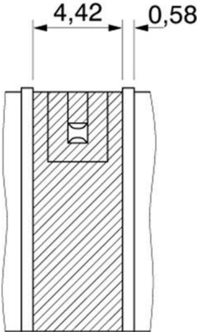
Dimensioned drawing
